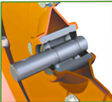
Hub HD type C2
